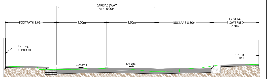
TYPICAL CROSS SECTION D-D SCALE 1:50
