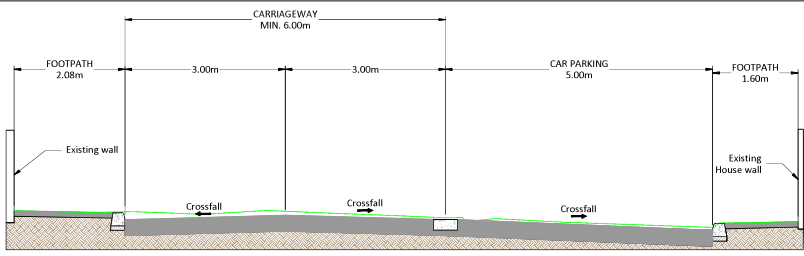
TYPICAL CROSS SECTION C-C SCALE 1:50
